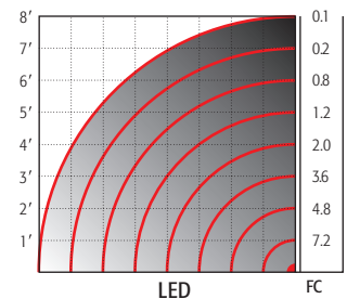
Horizontal Foot Candle Quarter Beam Spread
