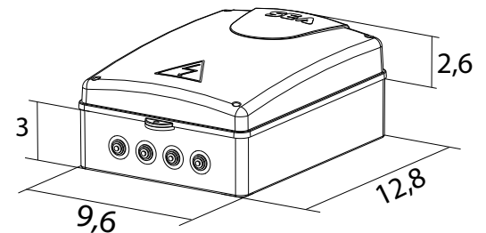
Dimensions (inches)
