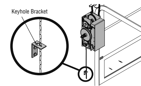
MANUAL DISCONNECT FOR MODELS MJ
