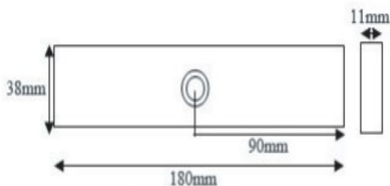
Electromagnetic lock
