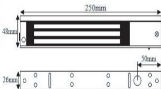
Electromagnetic lock
