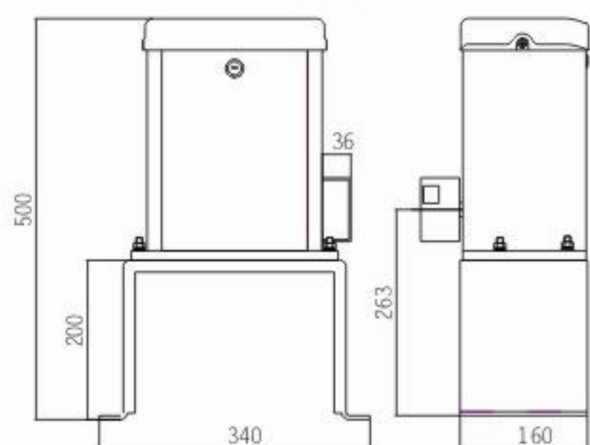
FAS-SLIDECH300BBUP Outline View
