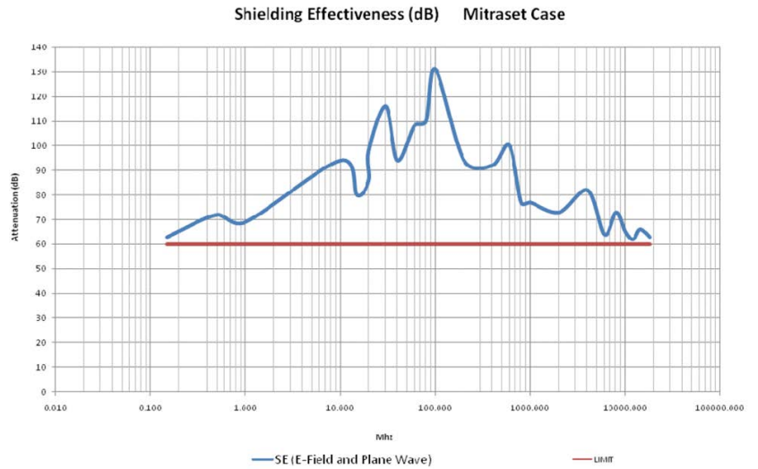
Mitraset Racklite Series with rubber corner
