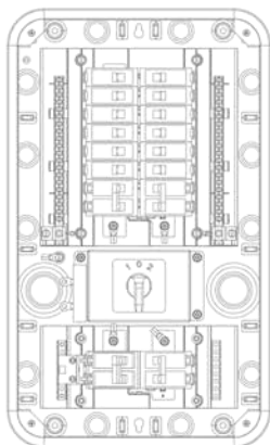
Figure 4.1 Disconnect
