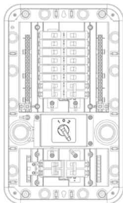
Figure 4.2 Machine power
