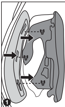
REMOVE THE CHEEK PADS
