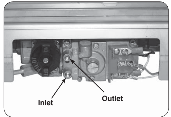
Fig. 19-1 12 valve: check pressure
