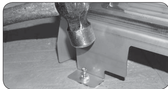
Fig. 16-2 Install hammer screws
