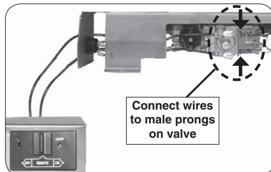
Fig. 15-3 Connect remote receiver to valve
