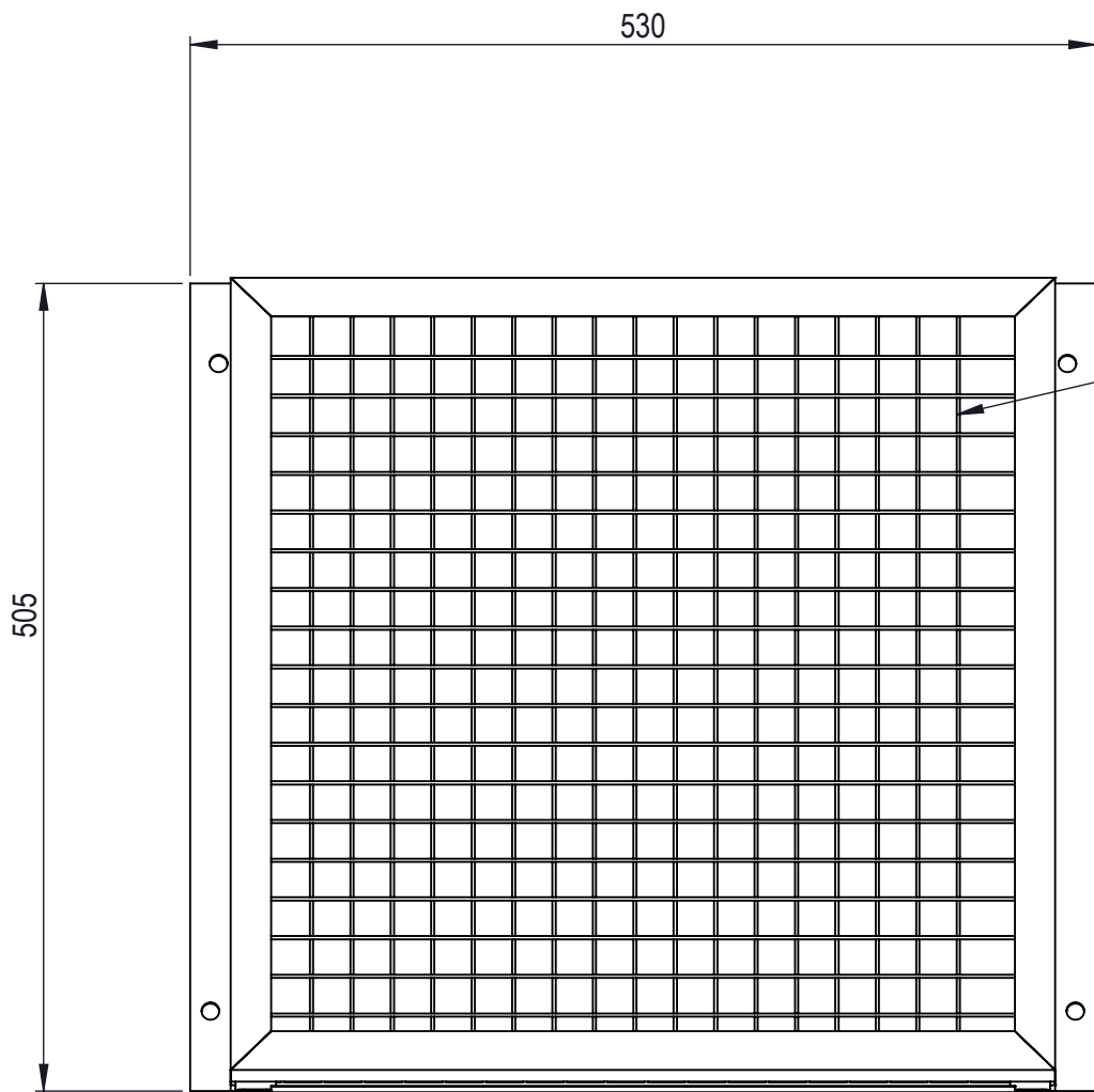
FRONT VIEW
