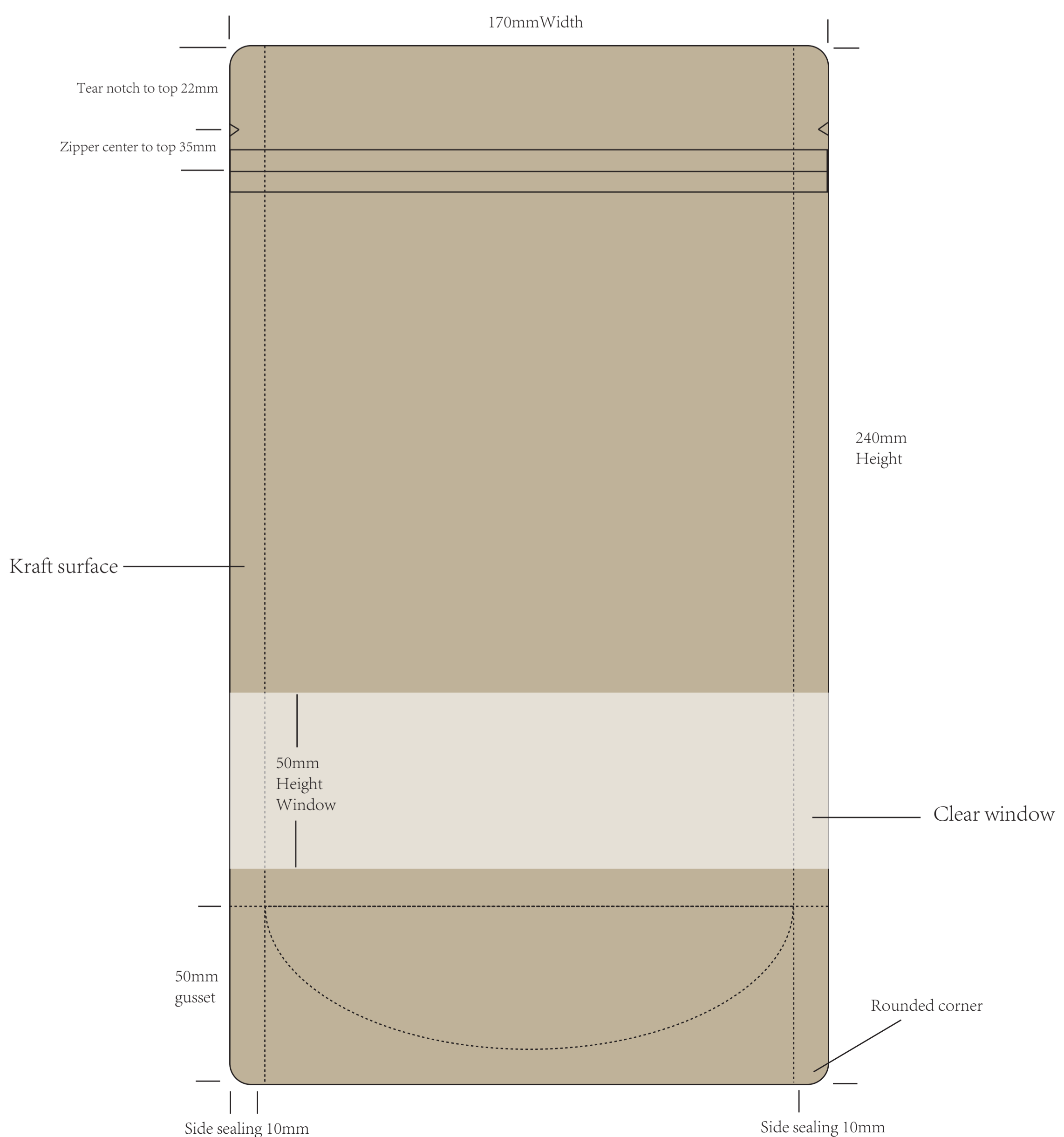
Size 3: 170mmWidth*295mmHeight*(50mm+50mm)Bottom gusset
