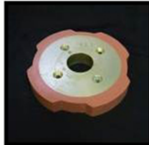
Rotary 7 D: 8.0" W: 1.2"
