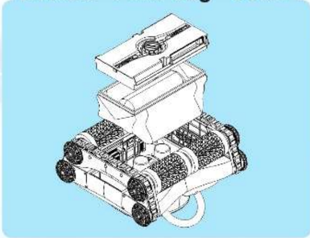
Bottom - Filter Bag - Cover
