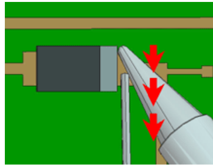
Soldering Chip Parts
