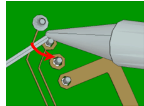
Point Soldering
