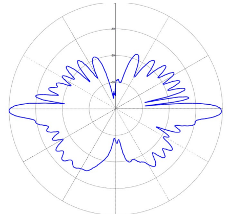
Vertical, 0° downtilt
