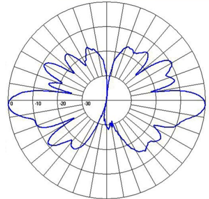
Vertical, 0° downtilt
