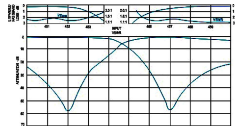
Span 10 MHz Response curve (typical), 5MHz Sep.
