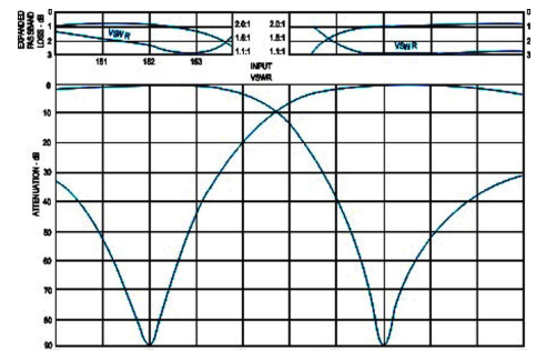
Response curve (typical), 5MHz Sep.
