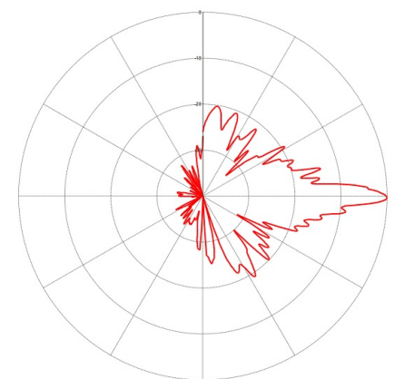
Vertical - 0° downtilt
