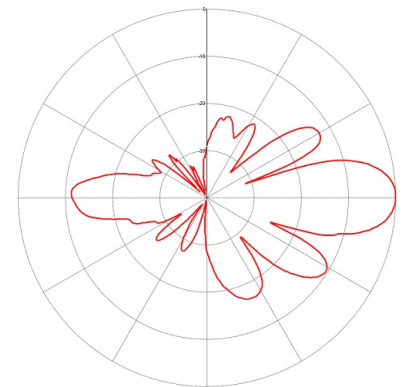
Vertical - 0° downtilt
