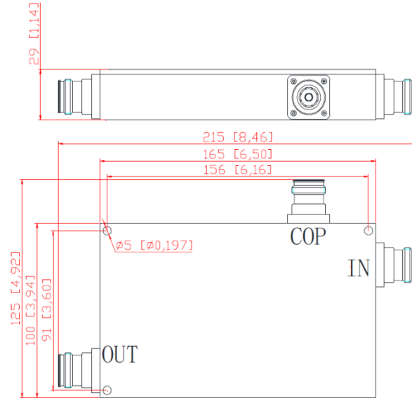
DDC240-(xx)-L4F, 4.3-10 female connector models
