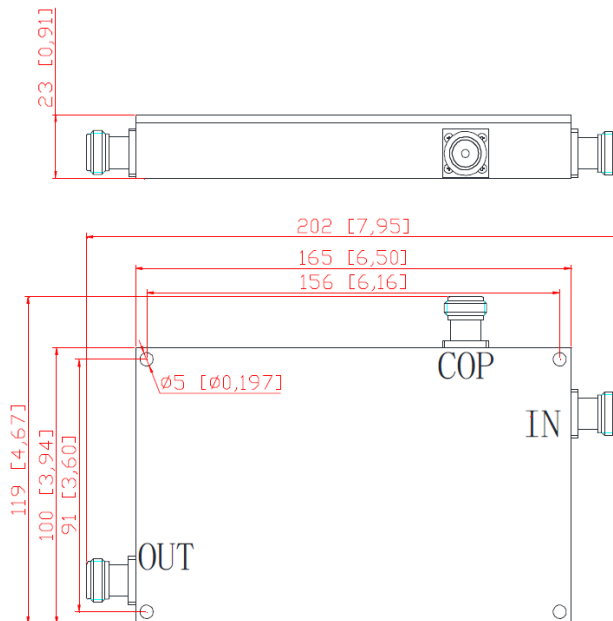
DDC240-(xx)-LNF, N female connector models
