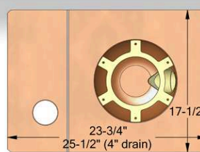
Bottom Outlet Roof Drain w/ Overflow ICC-ES PMG-1212
