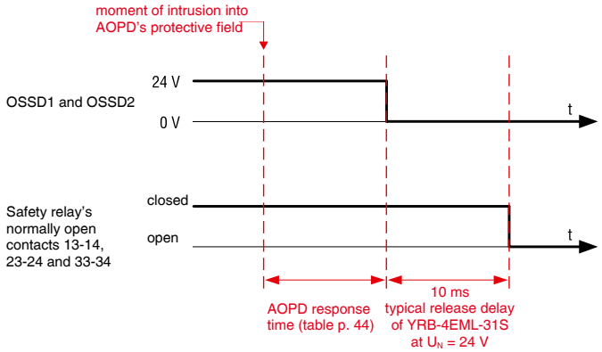
FIG. 28: SEQUENCE OF RELAY SWITCHING OPERATION
