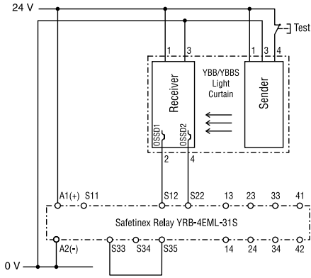
FIG. 30: CONNECTION DIAGRAM FOR AUTOMATIC RESTART MODE
