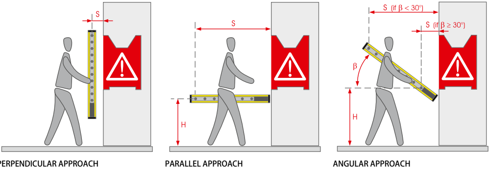
FIG. 5: MINIMUM SAFETY DISTANCE (EU)
