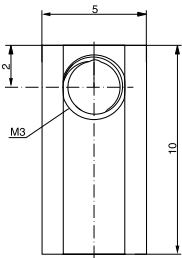
FIG. 23.1: TOP AND BOTTOM OPTIONAL MOUNTING BRACKET No. 7 (REF: YXW-0007-000)
