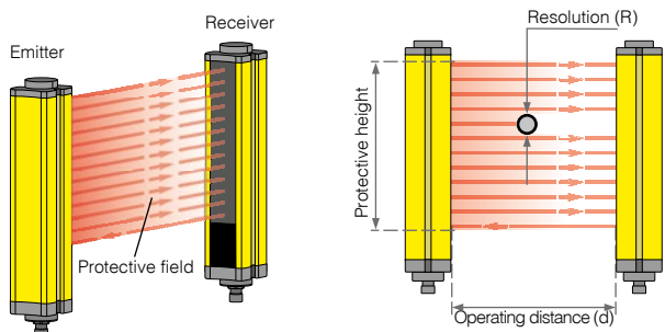
FIG. 2: OPERATING PRINCIPLE
