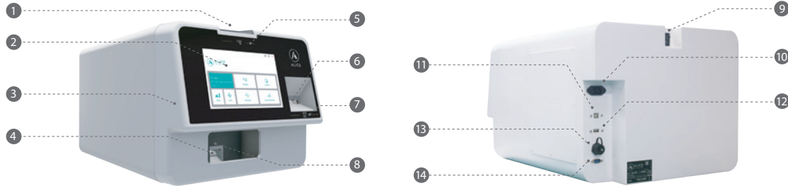
1. Coin entry 2. Screen / touch screen 3. Machine door 4. Coin exit 5. Led for active currency validator 6. Banknote entry and exit 7. Led for active banknote validator 8. Hidden lock for opening the door 9. Button for connecting the machine [ON/OFF], 10. Power cable input 11. OTG cable connector 12. USB cable connector 13. Ethernet connector 14. RS232 service connector
