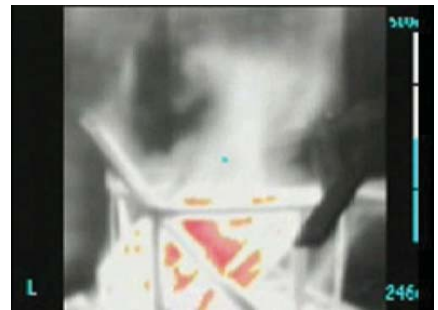
Low Sense image detail with Heat Seeker enhances heat source with red isotherm
