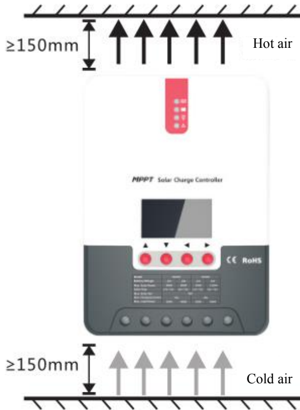
Fig. 2.1 Installation and heat dissipation
