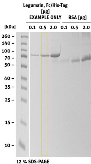
SDS-PAGE/Coll.Coomassie
