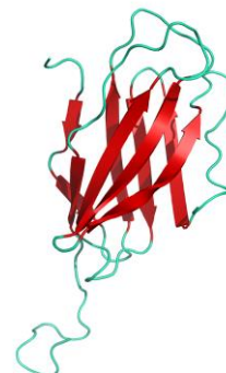
Structural model of human CTLA-4
