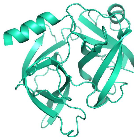
Structural model of the CELA3A protein (Example: porcine pancreatic elastase, pdb code:1BMA).
