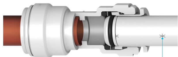
Pipe mark not level with collet head – indicating pipe not pushed fully home
