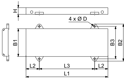
Fig. 80 EN/ISO base frame with 4 mounting holes
