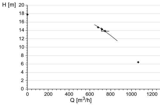
Fig. 71 Measured values for flow and head
