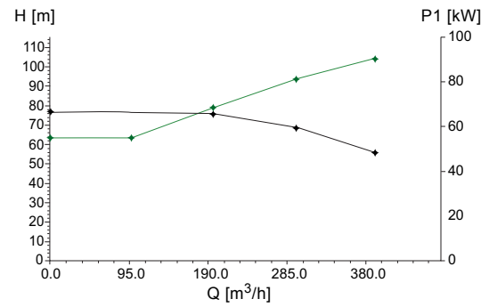
Fig. 76 Measured values for tested pump
