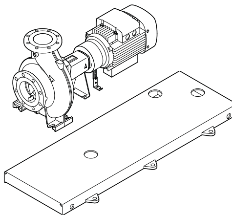
Fig. 46 Base frame prepared for grouting
