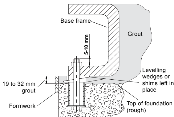
Fig. 48 Sectional view of foundation with anchor bolt, grouting and base frame
