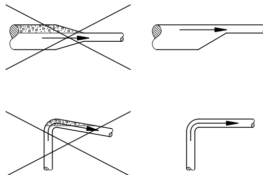
Fig. 49 Pipelines
