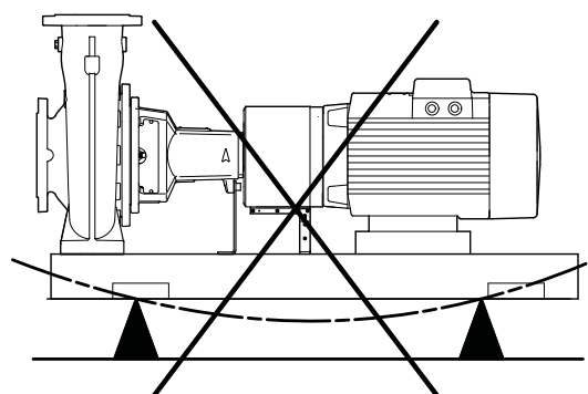
Fig. 45 Incorrect foundation
