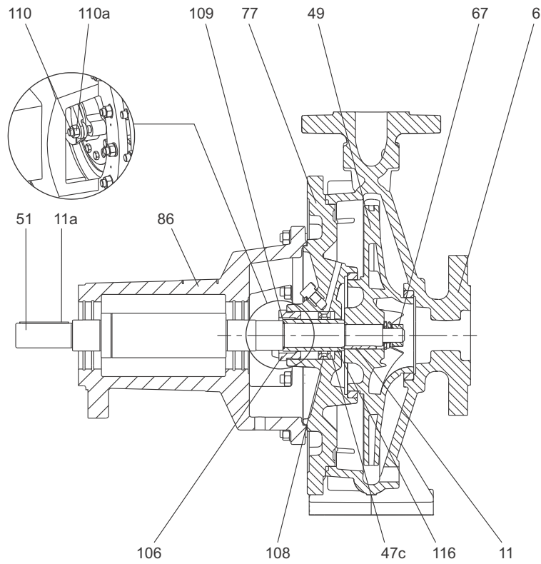
Fig. 10 Sectional drawing, stuffing box, single cover
