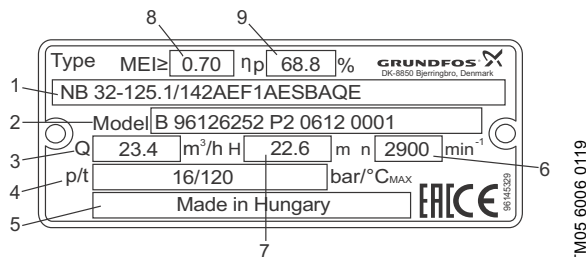
Fig. 5 Example of nameplate
