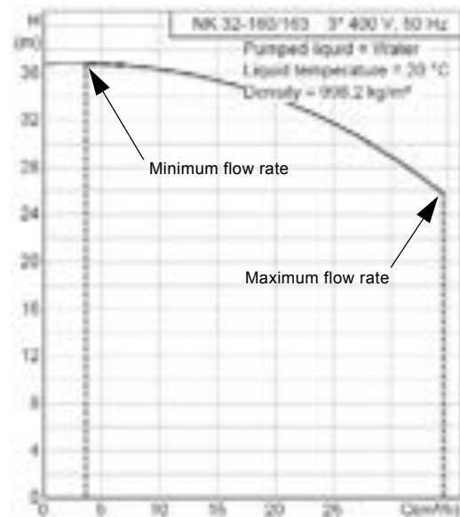
Fig. 36 Example from Grundfos Product Center showing minimum and maximum flow rate
