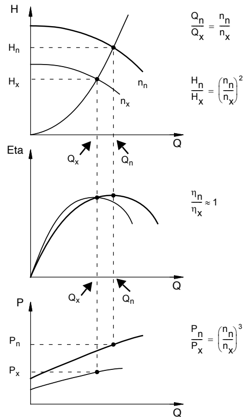
Fig. 60 Affinity equations
