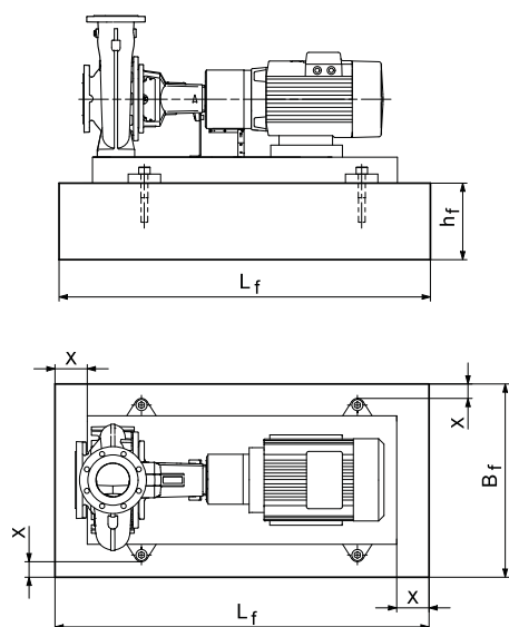
Fig. 43 Foundation, X is equal to minimum 100 mm
