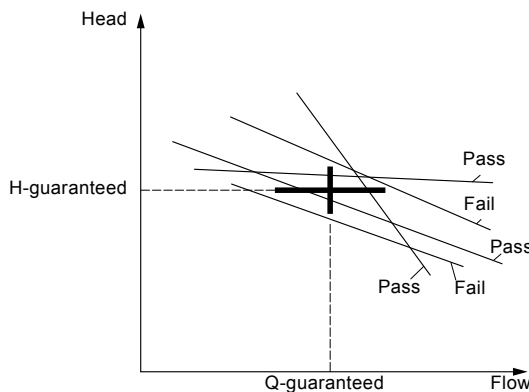
Fig. 68 Pump curves that either pass or fail to cross the tolerance cross of the guarantee point
