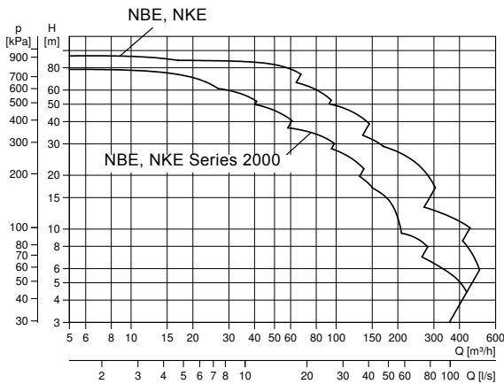
Fig. 55 E-pumps performance range
