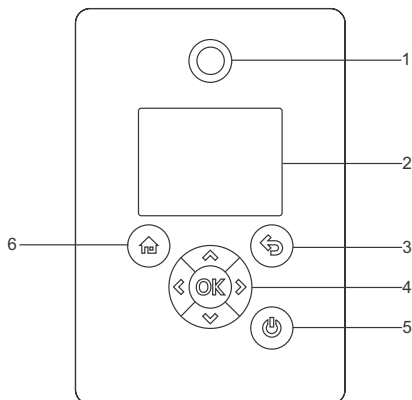
Fig. 61 Advanced control panel
