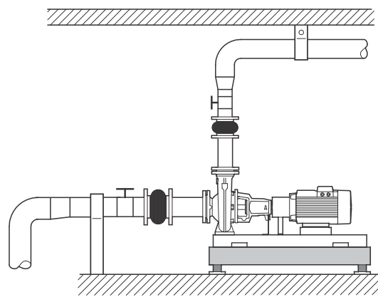
Fig. 50 Pipeline mounting
