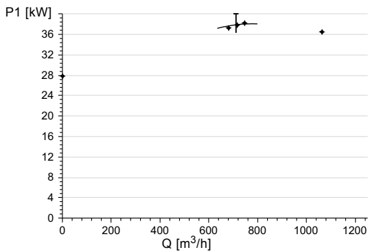
Fig. 72 Measured values for consumed power
