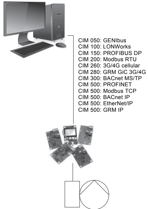
Fig. 64 Structure of a central building management system
