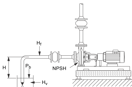
Fig. 41 Suction lift with positive H
