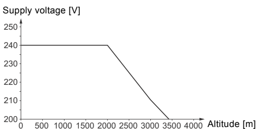
Fig. 35 Supply voltage for single-phase motor in relation to altitude
