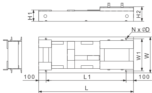
Fig. 84 C-channel base frame with 4 mounting holes
