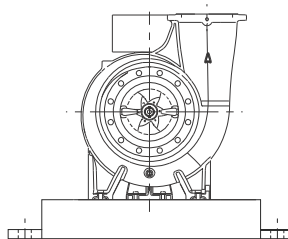
Fig. 26 Schematic view of NK pump mounted on an EN/ISO base frame
