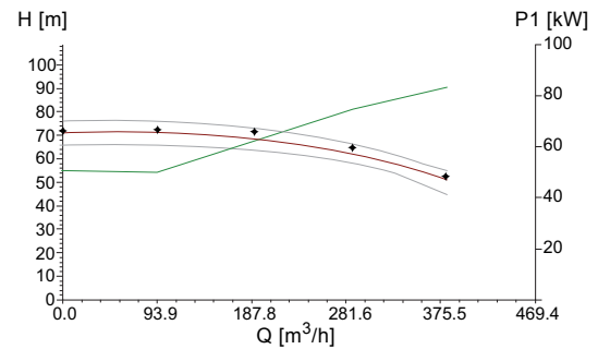
Fig. 77 The values in fig. 76 calculated to a reference speed for comparison to a reference performance
