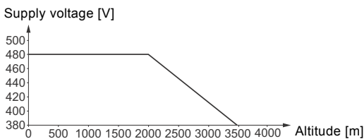
Fig. 34 Supply voltage for three-phase motor in relation to altitude
