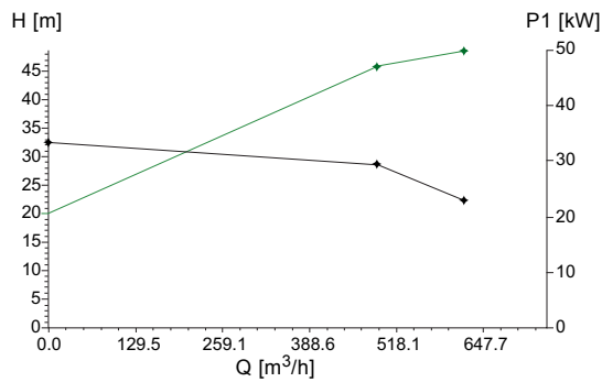
Fig. 74 Measured values for tested pump
