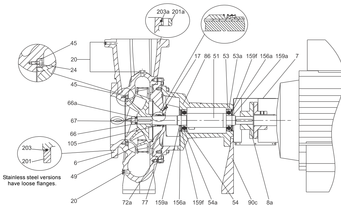
Fig. 9 Sectional drawing, with tangential outlet, DN 200 and DN 250
