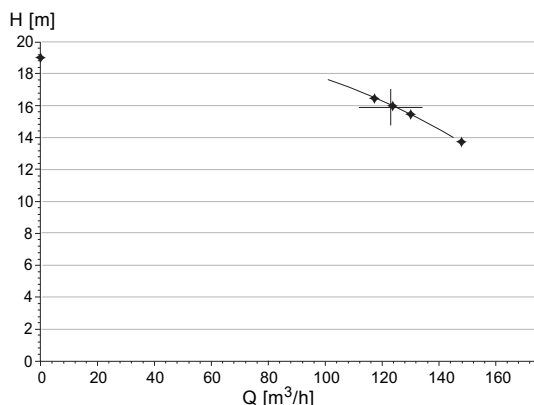
Fig. 67 Five measured test points are used to verify one guarantee point
