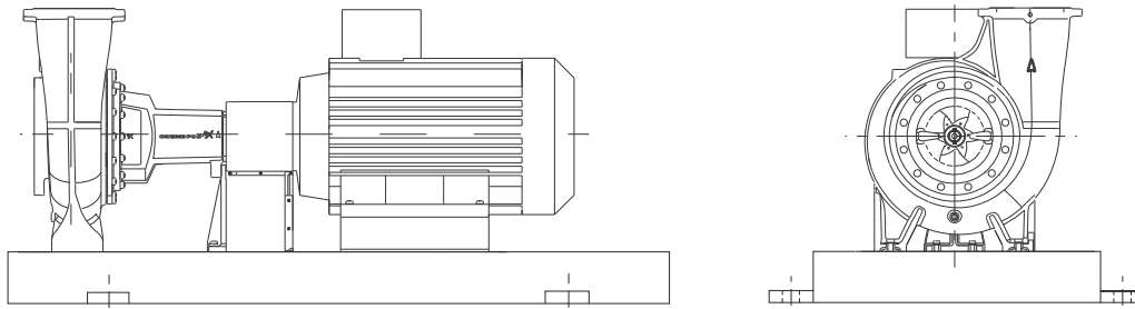
Fig. 78 NK pump with EN/ISO base frame
