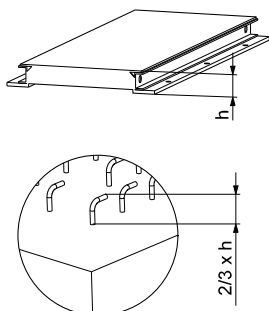
Fig. 47 Reinforcing steel bars embedded in foundation
