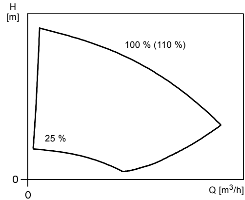
Fig. 56 Duty range of E-pumps
