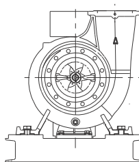
Fig. 27 Schematic view of NK pump mounted on a C-channel base frame
