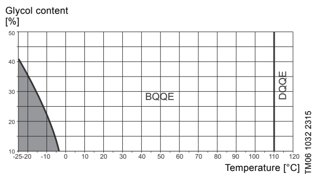
Fig. 37 Operating range of EPDM shaft seals
