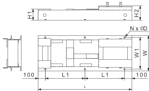
Fig. 85 C-channel base frame with 6 mounting holes
