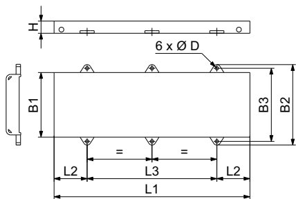
Fig. 81 EN/ISO base frame with 6 mounting holes
