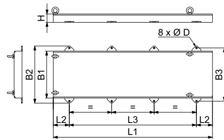
Fig. 83 EN/ISO base frame with 8 mounting holes
