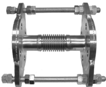
Fig. 54 Metal bellows expansion joint with limiting rods
