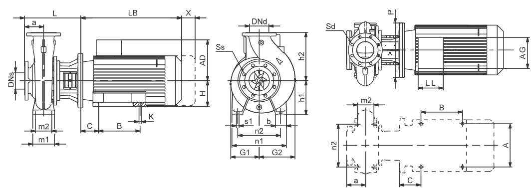
Mounting design C1, centre outlet
