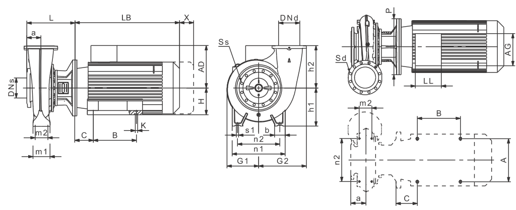
Mounting design C2, tangential outlet
