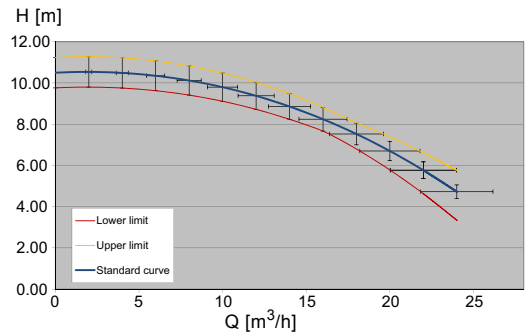
Fig. 73 Q-H curve with tolerance crosses on complete performance range
