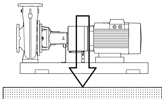
Fig. 44 Correct foundation
