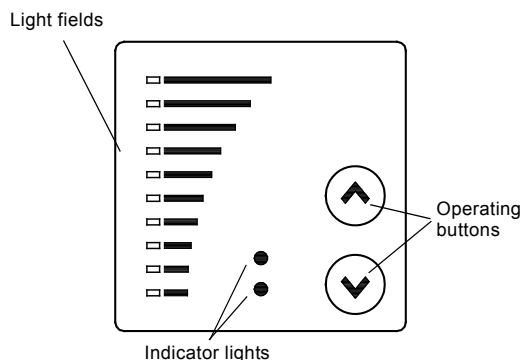
Fig. 62 Operating panel for 15-22 kW, 2-pole and 11 - 18.5 kW, 4-pole motors
