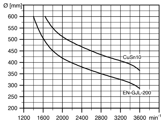
Fig. 58 Maximum permissible speed
