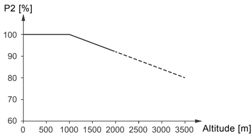
Fig. 33 Motor output power in relation to altitude
