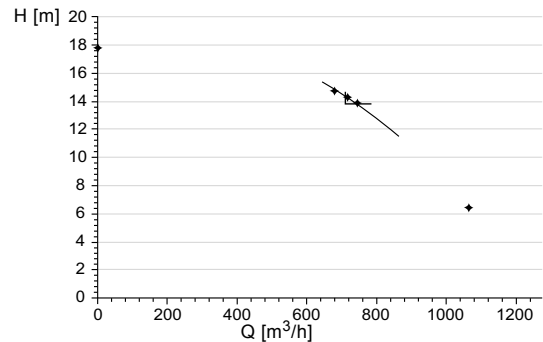
Fig. 69 Measured values for flow and head
