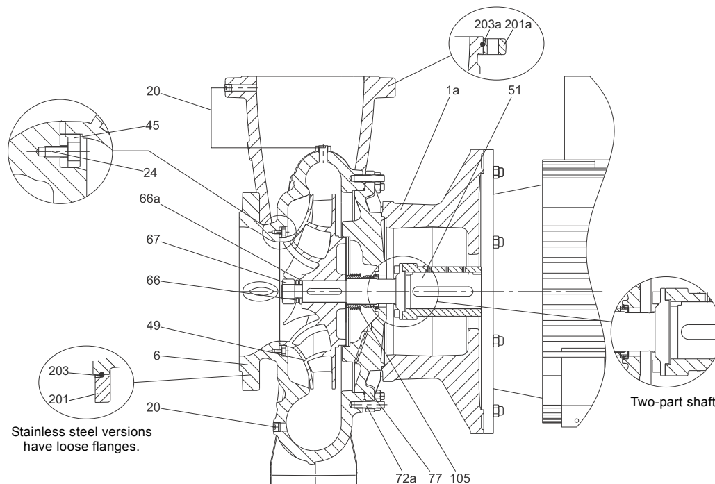
Fig. 7 Sectional drawing, tangential outlet, DN 200 and DN 250
