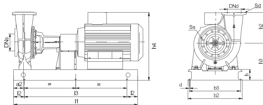
Fig. 87 NK pump with C-channel base frame
