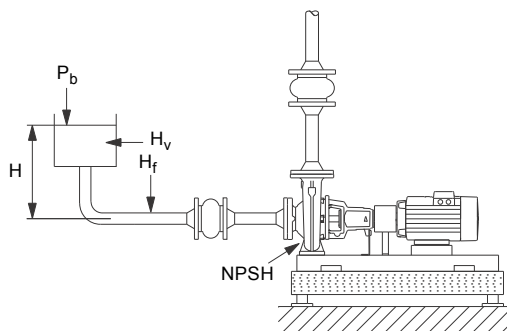
Fig. 42 Suction lift with negative H
