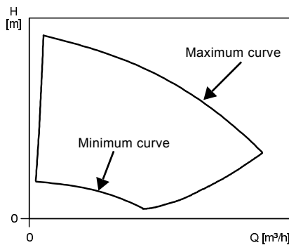
Fig. 59 Minimum and maximum performance curves
