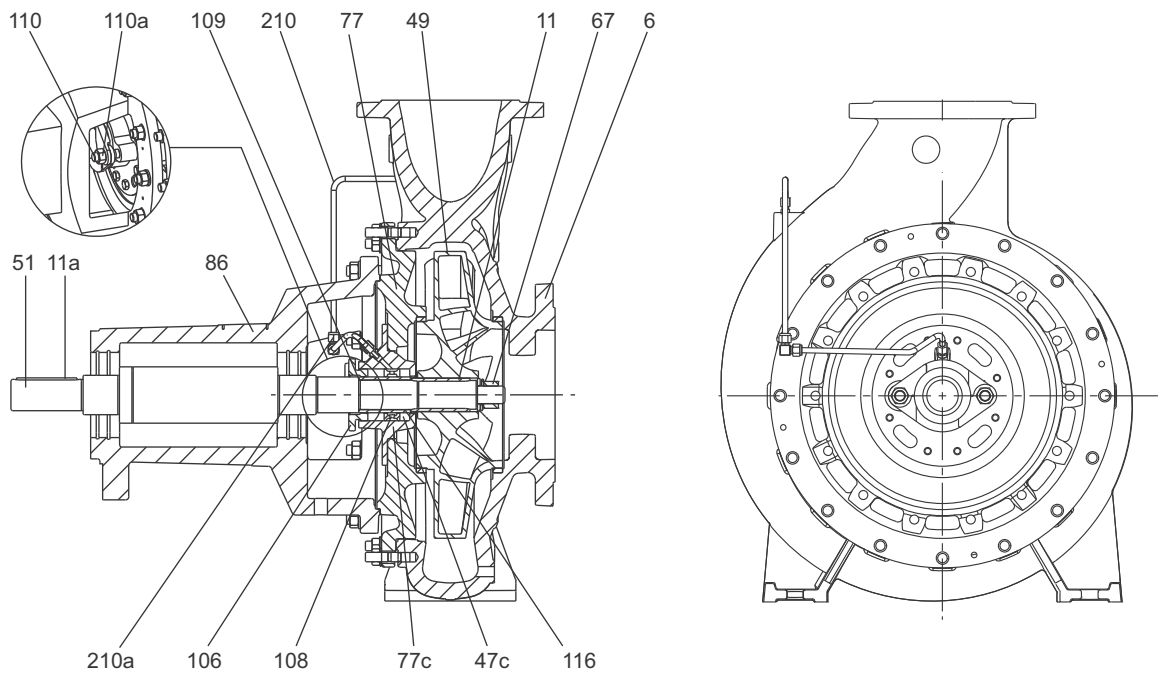
Fig. 11 Sectional drawing, stuffing box, split cover
