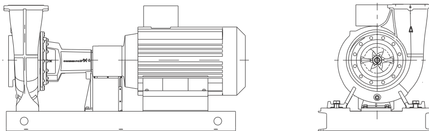
Fig. 79 NK pump with C-channel base frame
