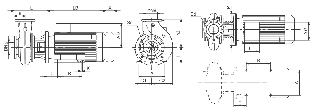
Mounting design B
