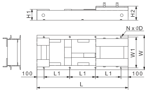
Fig. 86 C-channel base frame with 8 mounting holes
