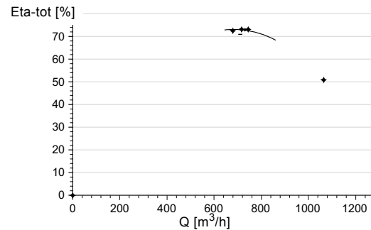
Fig. 70 Measured values for total efficiency
