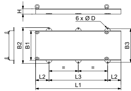
Fig. 82 EN/ISO base frame with lifting eyes and 6 mounting holes
