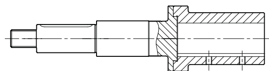
Fig. 22 2-part stub shaft, NB pump
