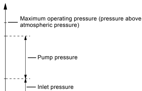
Fig. 39 Pressures in the pump
