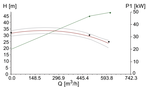
Fig. 75 The values in fig. 74 calculated to a reference speed for comparison to a reference performance curve
