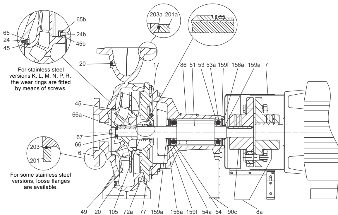
Fig. 8 Sectional drawing, centre-line outlet
