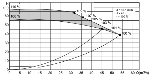
Fig. 57 Example on extended performance range up to 110 % as a part of the operation range
