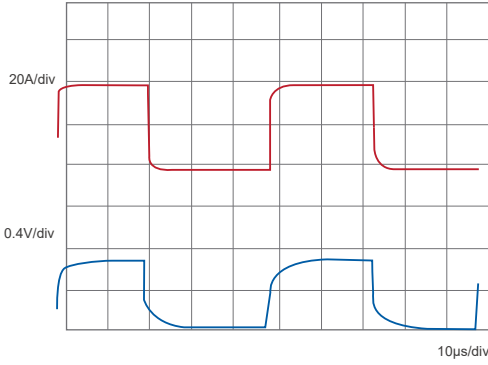
Output Wave-2
