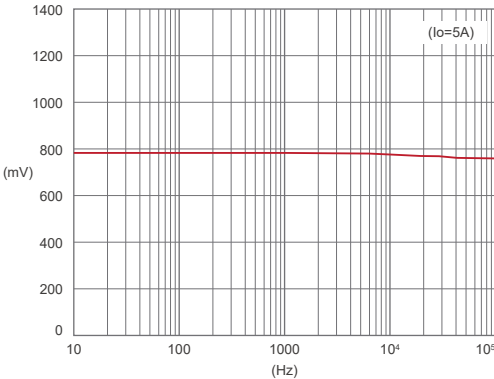
Frequency Characteristic
