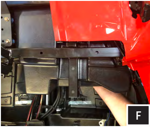
F. Lift the enclosure into place. Using the factory glove box mounting hardware, fasten the enclosure into place. Pull sub enclosure wiring towards the center of the vehicle to avoid being pinched by the chassis.
