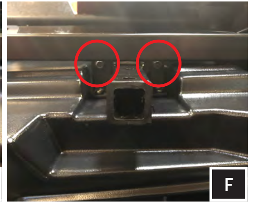
F. Lift the enclosure into place. Using the factory glove box mounting hardware, fasten the enclosure into place. Pull sub enclosure wiring towards the center of the vehicle to avoid being pinched by the chassis.
