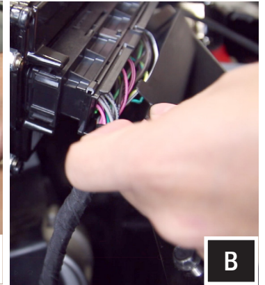
B. Tilt the brain back, unsnap the perimeter of the connector cover as it will be replaced by the provided cover that has a cable relief cut-out.
