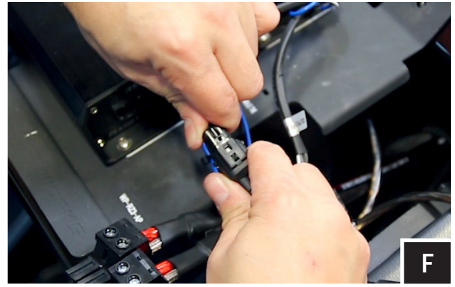
F. Connect the B-H1909 speaker harness to the 300.4 amplifier front output.
