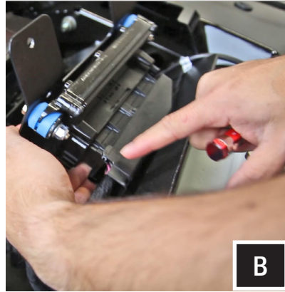
B. Tilt the brain back, unsnap the perimeter of the connector cover as it will be replaced by the provided cover that has a cable relief cut-out.
