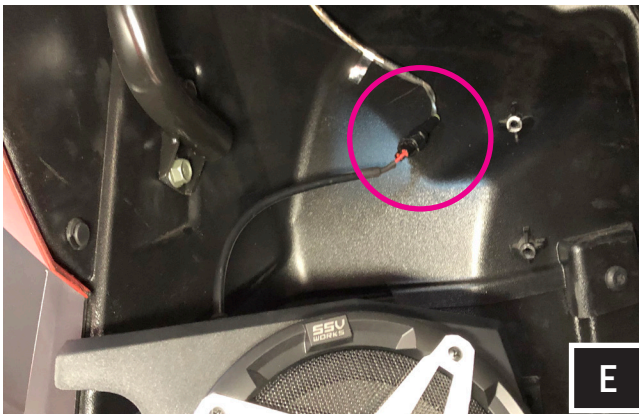
E. Connect the B-H1909 cable to the speaker pod and zip tie all cables to the frame.
