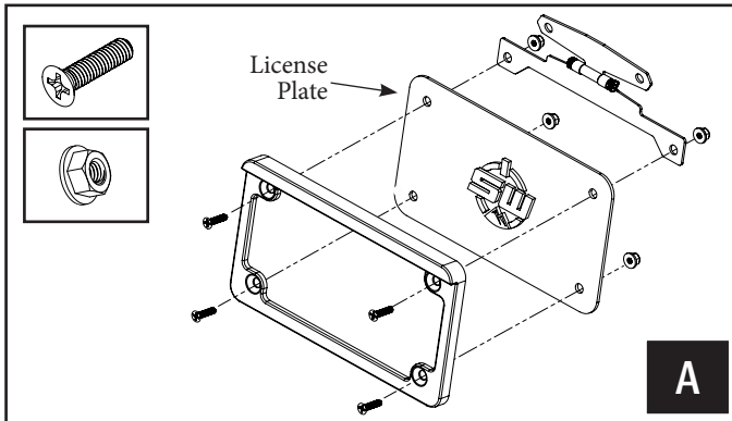
A. Use (4) M4 Phillips flat head screws and flanged locknuts, included in the kit, to assemble the license plate between the license plate frame and bracket as shown above.
