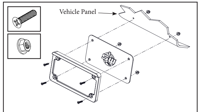
The license plate frame can also be mounted directly to the vehicle panel without using the provided adjustable bracket. Use the (4) M4 Phillips flat head screws and flanged locknuts, included in the kit, to secure the license plate frame to the vehicle.
