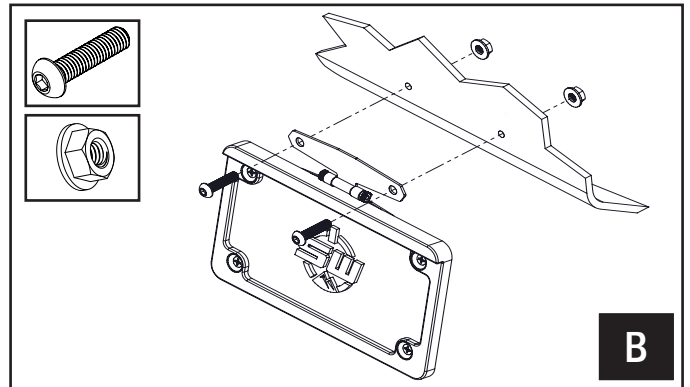
B. Use the button head Allen screws and flanged locknuts, included in the kit, to secure the license plate frame bracket to the vehicle.
