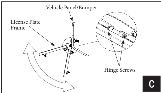
C. The license plate frame bracket has a 240° up and down adjustability for various mounting options such as above bumper, vertical body mounting or under bumper mounting. Tighten the 3mm bracket hinge screws to lock the angle (see inset above).
