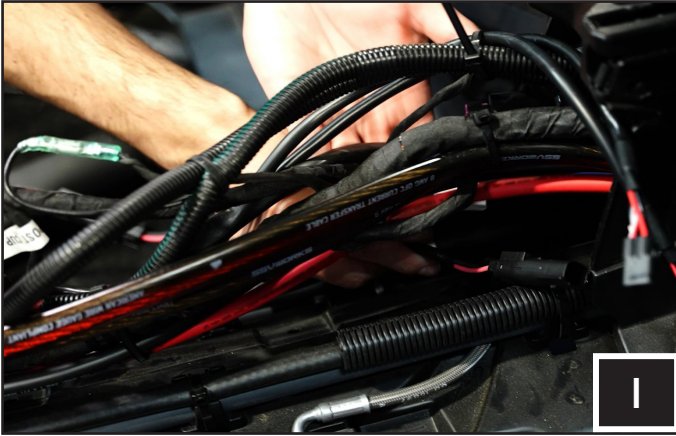
I. Use zip ties to tidy up the install.
