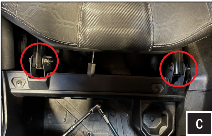
C. Remove the (2) 13mm bolt and nut on the front seat rail.
