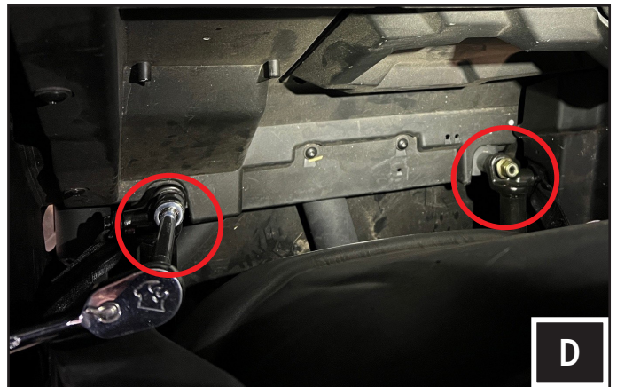
D. Slide the seat forward and remove the rear 18mm seat rail nuts.
