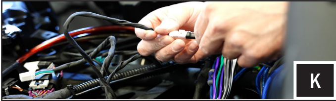
K. Plug in the 8-pin speaker and 2-pin subwoofer input connectors of the amplifiers to the factory radio output wiring.
