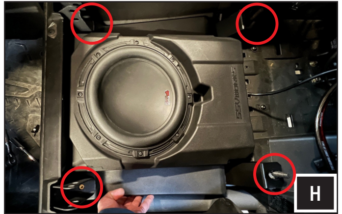
H. Slide the Mav R subwoofer enclosure under the front seat rail mounts and insert the brackets to the rear seat rail studs.
