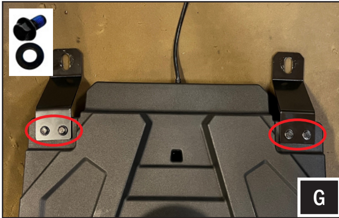
G. Mount the brackets on the Mav R subwoofer enclosure using (4) M6x12mm hex head bolts and washers.
