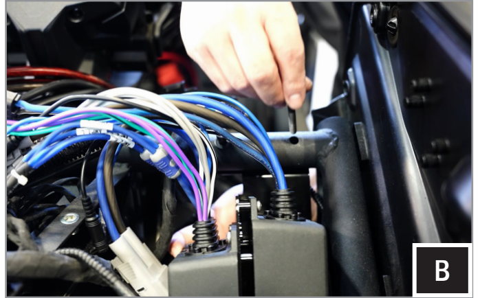
B. Bolt on the amp bracket to the chassis frame using (x3) B-S1287 M6-1x45mm socket head screw and B-W1052 washers.
