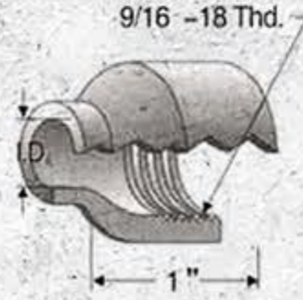
Alumina for Gas Lens 1"
