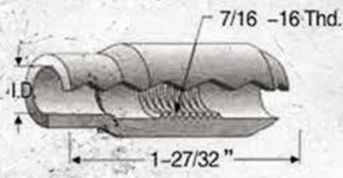
Alumina 1-27/32"
