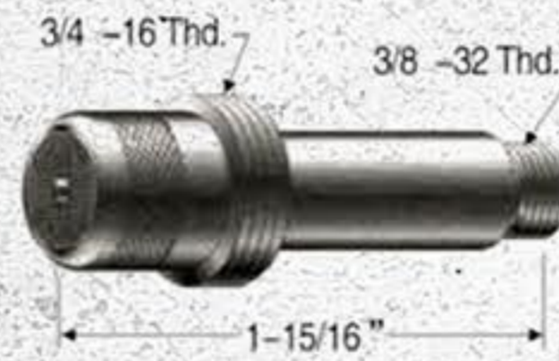
Gas lens
