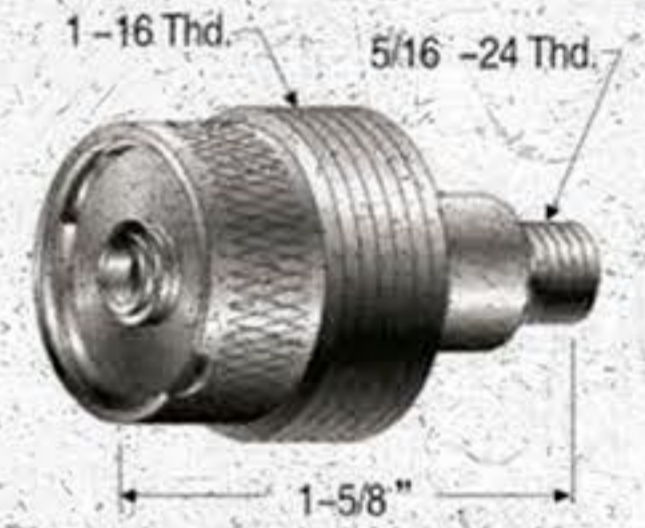
Extra large stubby gas lens
