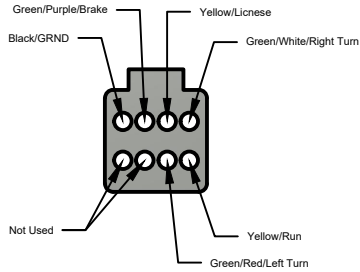
Back View of TYPICAL STOCK Male Main Bobber Connector
