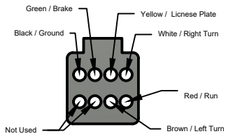
Back View of BROGUE Male Main Connector
