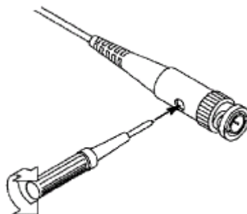
Fig. 4-6 Adjust Probe
