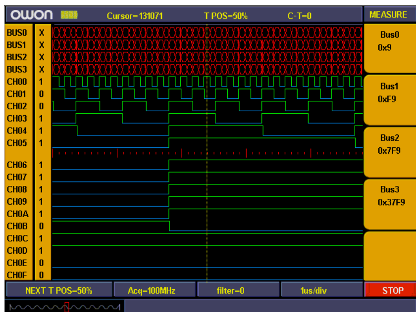
Fig.5-72: Bus measurement
