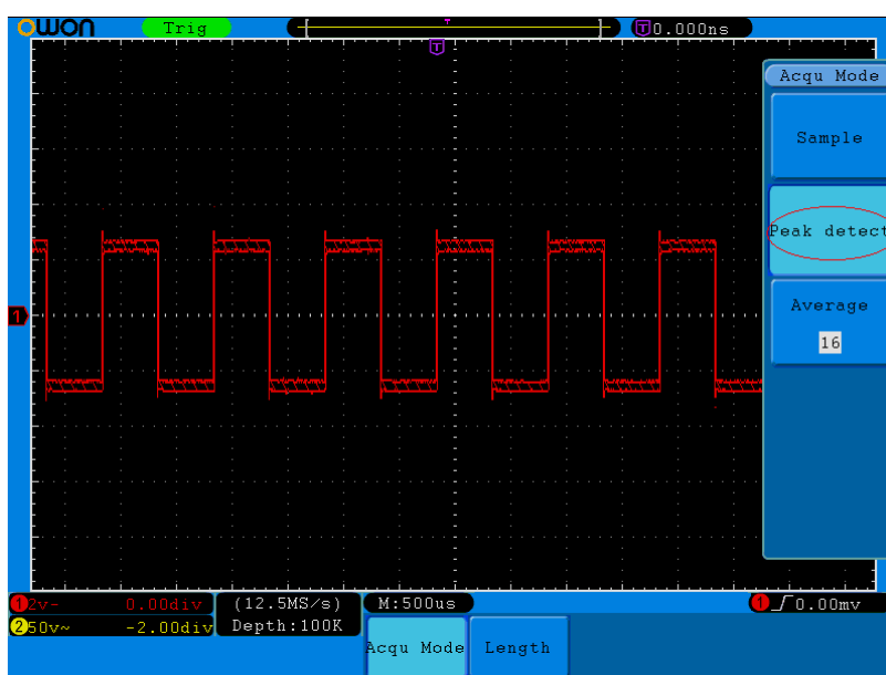
Figure 5-28 Peak Detect mode, under which the burrs on the falling edge of the square wave, can be detected and the noise is heavy.
