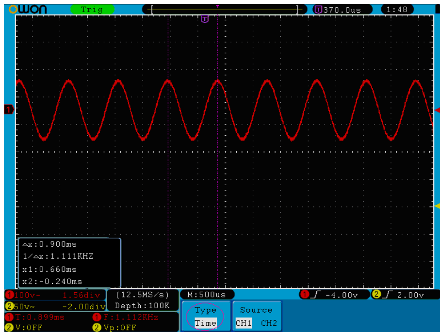
Figure 5-62 Waveform of Cursor Measurement
