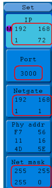
Figure 5-55 Set the network parameters of the oscilloscope
