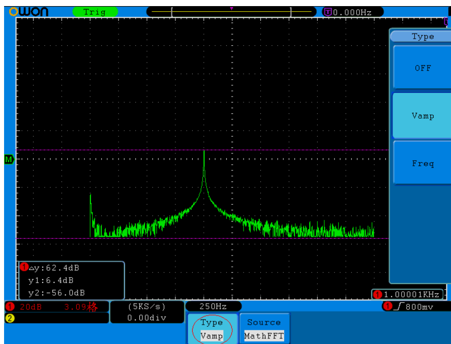
Figure 5-64 wave of Vamp cursor measurement
