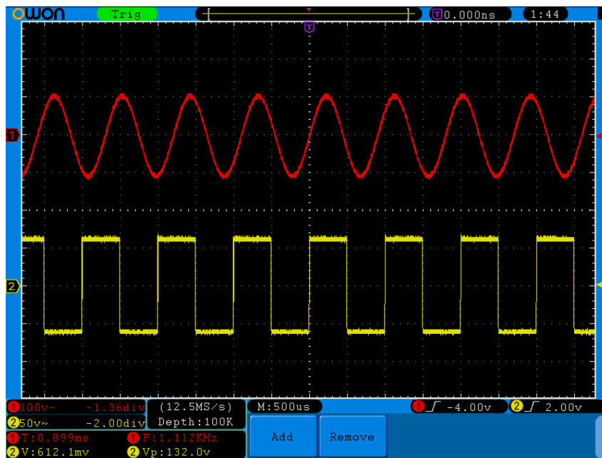
Figure 6-1 Measure Frequency and PK-PK value for a given signal
