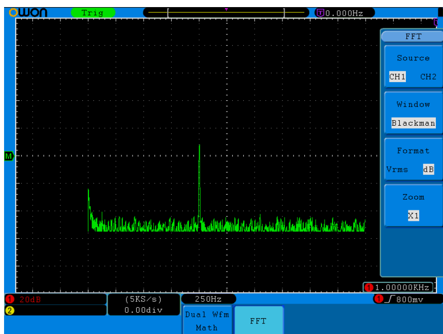
Figure 5-13 Blackman window
