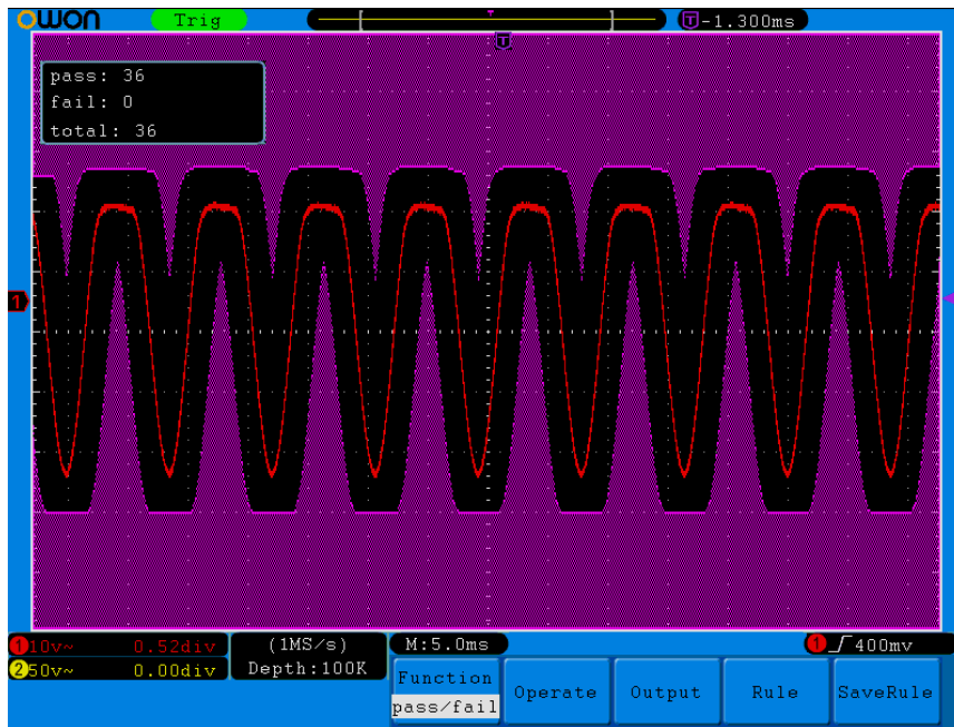
Figure 5-47 Pass/Fail test
