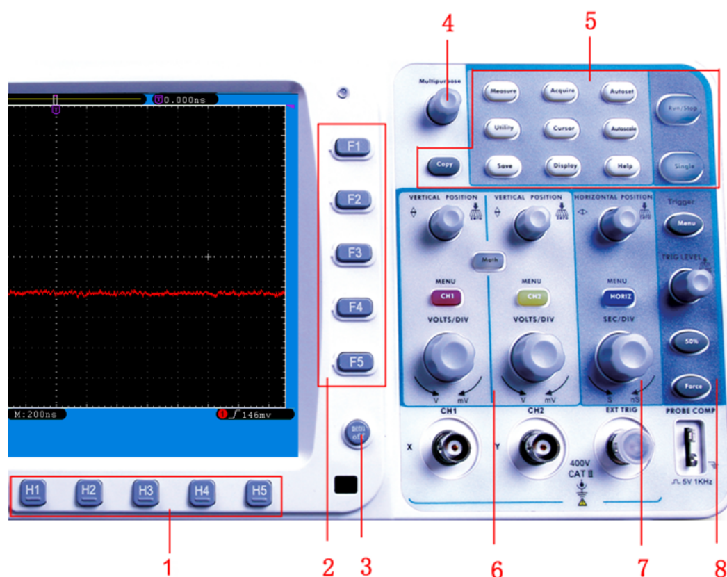
Figure 4-5 Keys Overview
