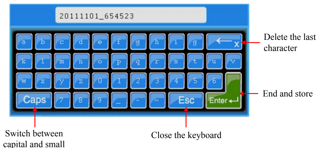
Figure 5-38 Edit the File Name
