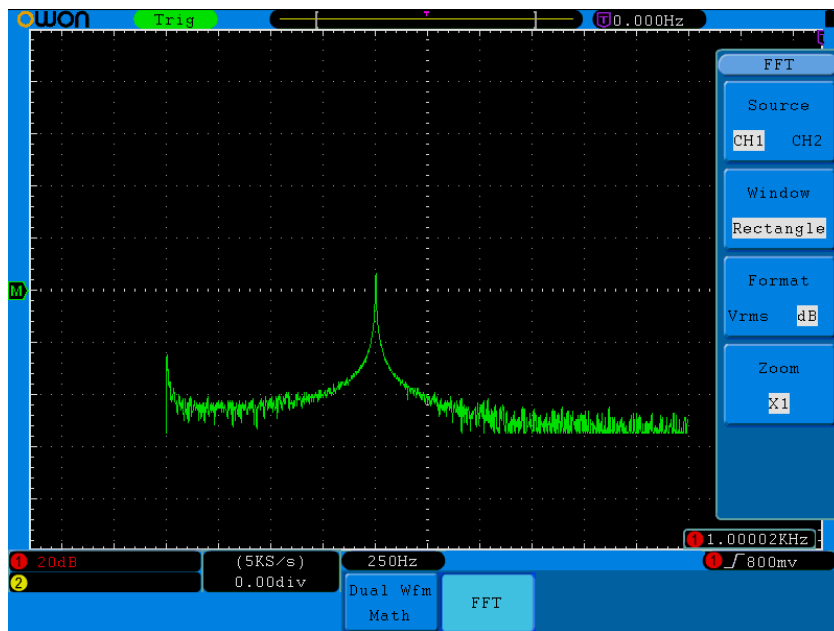
Figure 5-10 Rectangle window
