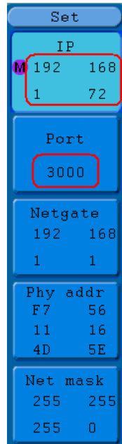
Figure 5-52 Set the network parameters of the oscilloscope
