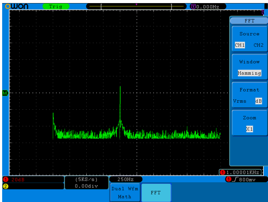
Figure 5-11 Hamming window
