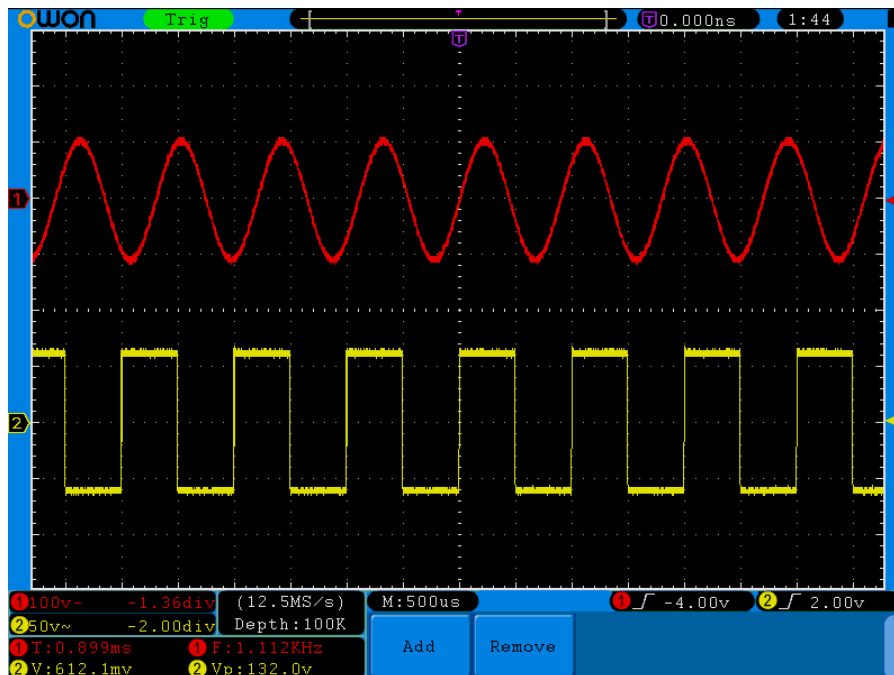
Figure 5-57 automatic measurement
