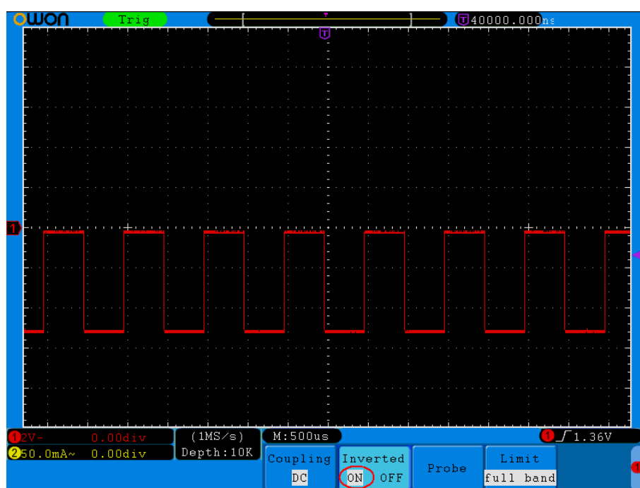
Figure 5-7 Inverted Waveform
