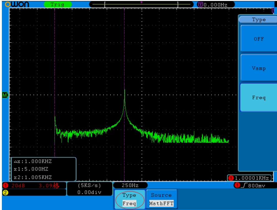
Figure 5-65 wave of Freq cursor measurement
