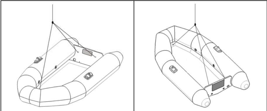
Lifting points for rigid keel boats
