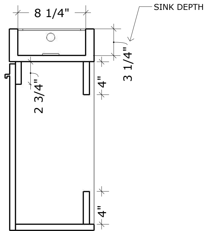
SECTION CUT
