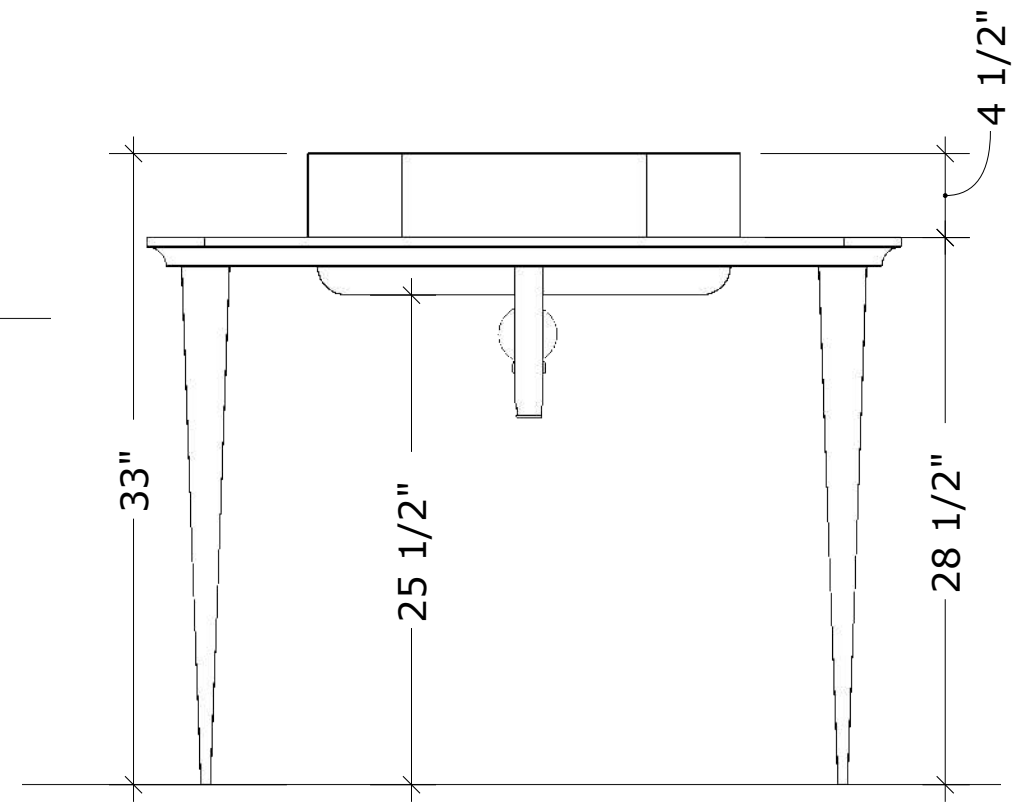
FRONT ELEVATION
