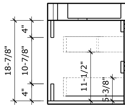
SECTION CUT
