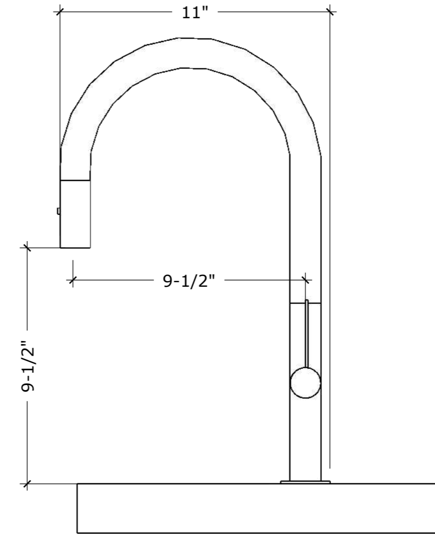
SIDE
