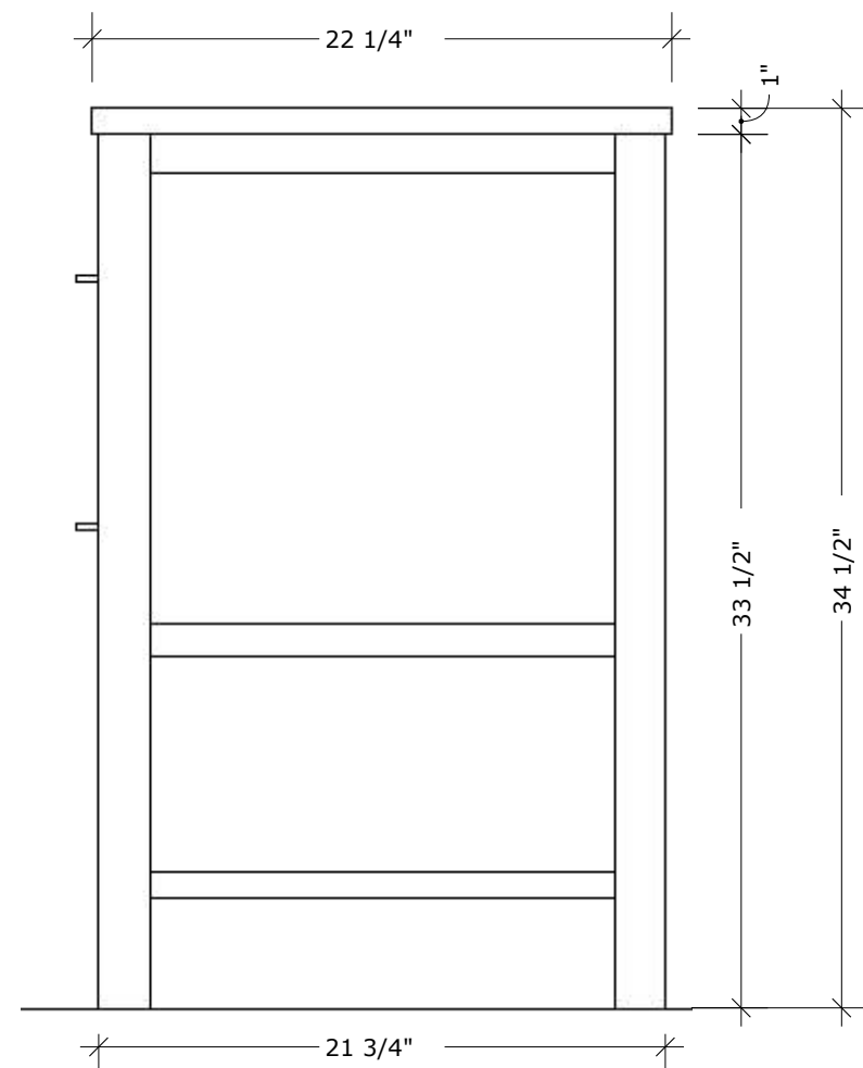
SIDE ELEVATION
