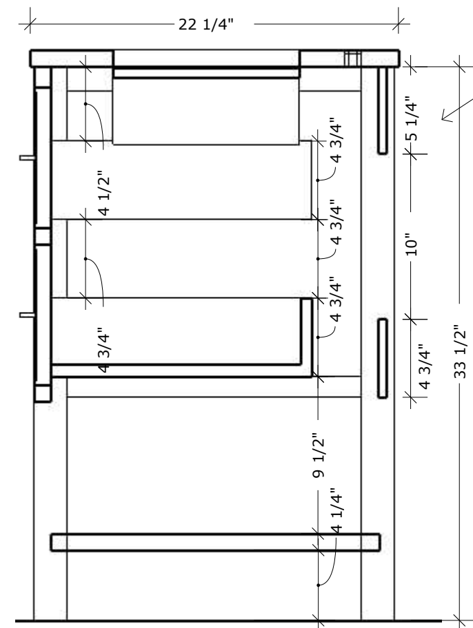
SECTION CUT
