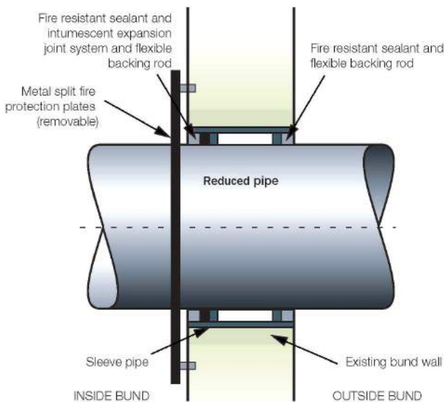
Figure 12.6 Sealed sleeve upgrade option (after HSE, 2009a)
