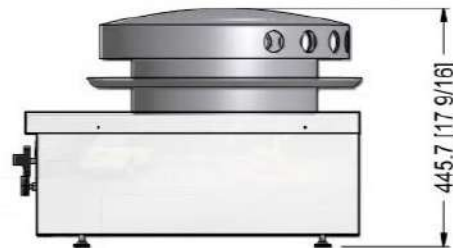
SIDE ELEVATION ( 1 : 10 )
