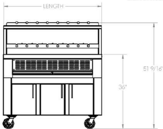
SHOWN: CP-CHU-FL-SF-48 WITH OPTIONAL SWIVEL CASTERS
