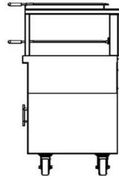
SHOWN: CP-CHU-FL-SF-48 WITH OPTIONAL SWIVEL CASTERS
