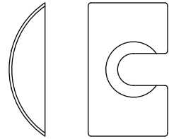
FF Half Moon Washer x 6 arandela de media luna x 6
