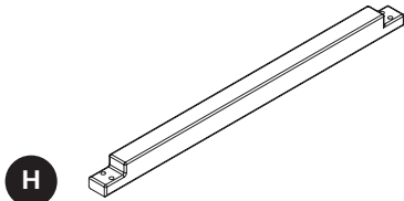
H Center Base Rail x 1 Barra base central x 1
